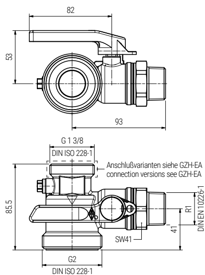
Anschlussadapter GZHEA Connecting adaptors GZHEA
