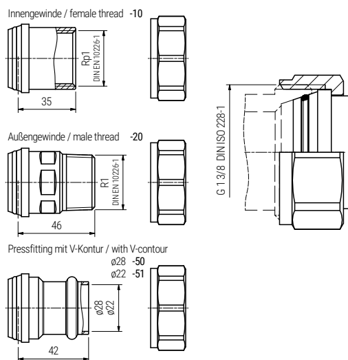
Anschlussadapter GZHEA Connecting adaptors GZHEA
