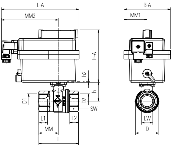
Maßskizze measured sketch
